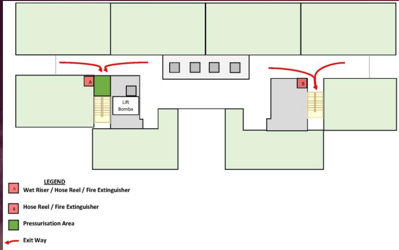
COMMON CORRIDOR EXIT PLAN TOWER B & D
