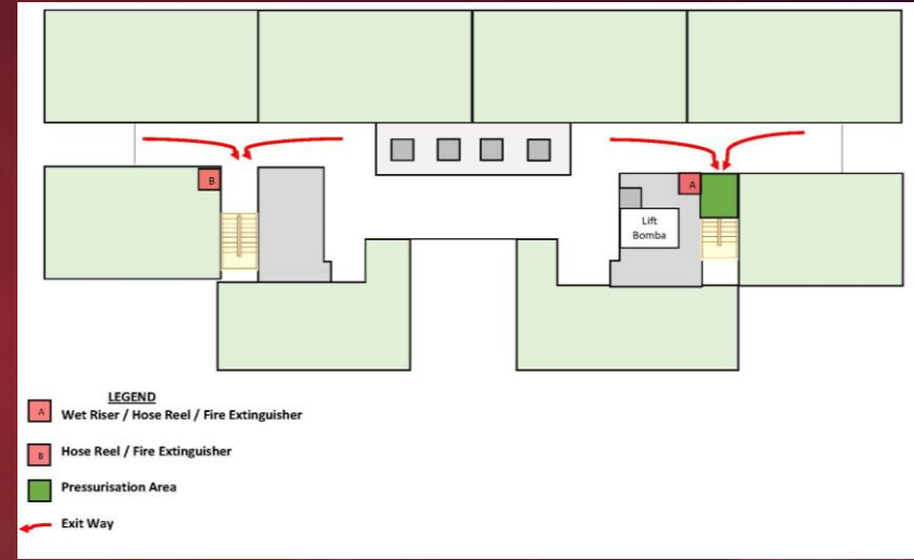
COMMON CORRIDOR EXIT PLAN TOWER A & C
