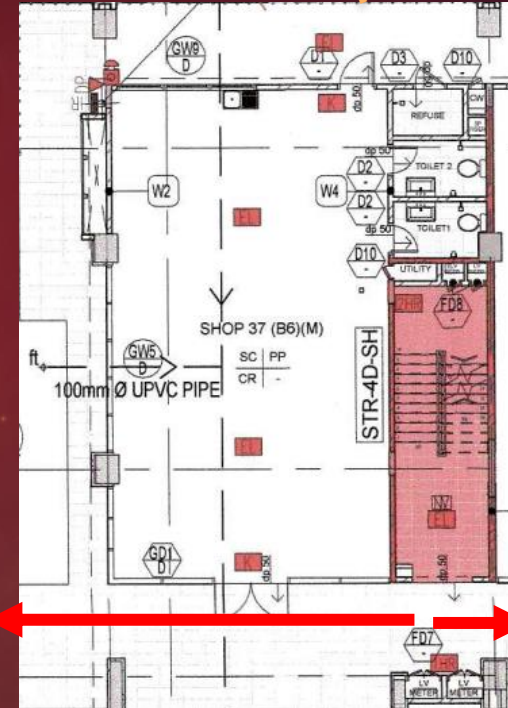
Common corridor exit plan for unit 27 - 43A (2 Floors)
